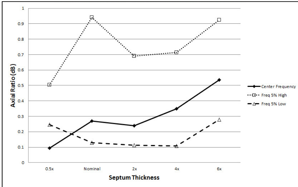
Figure 6: N2UO septum feed, sensitivity to septum thickness
