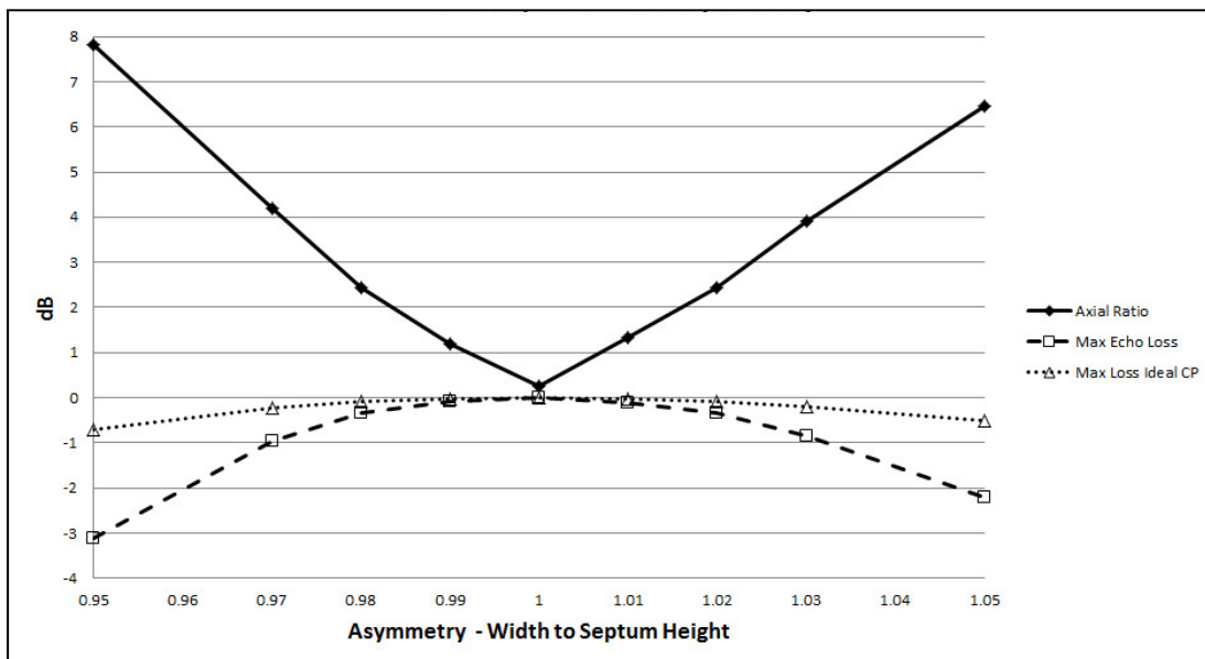
Figure 10: Effect of waveguide asymmetry on N2UO septum feed
