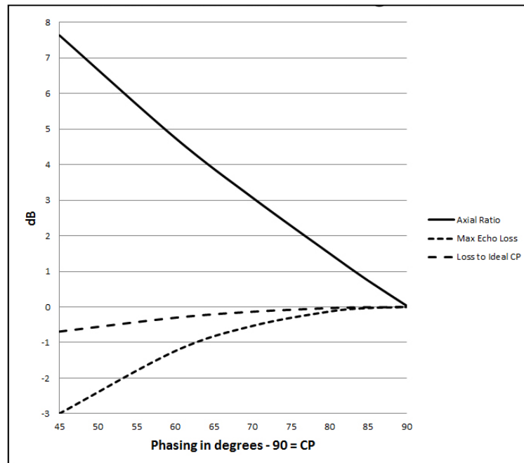
Figure 2: Circular Polarization phasing error and resultant losses
