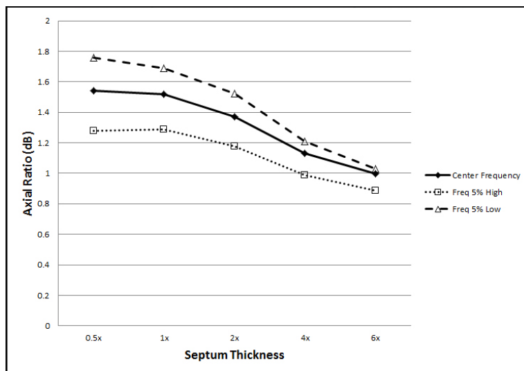
Figure 4: OK1DFC septum feed, sensitivity to septum thickness
