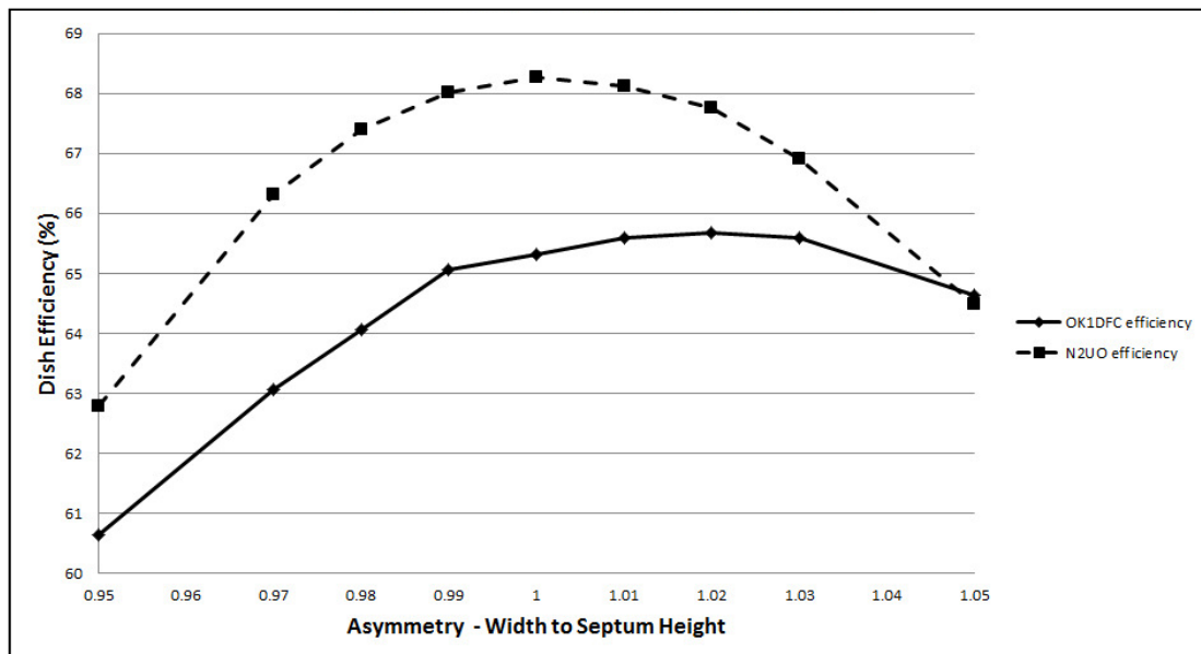
Figure 11: Effect of septum feed asymmetry on dish antenna performance
