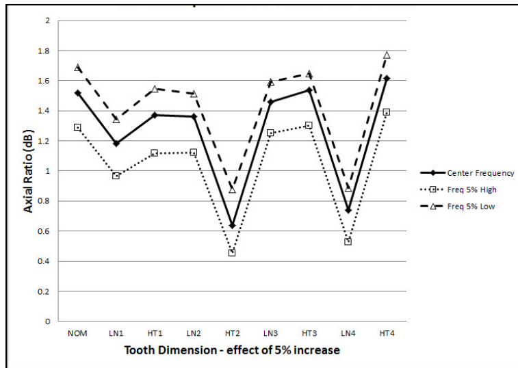
Figure 3: OK1DFC septum feed, sensitivity to tooth dimensions
