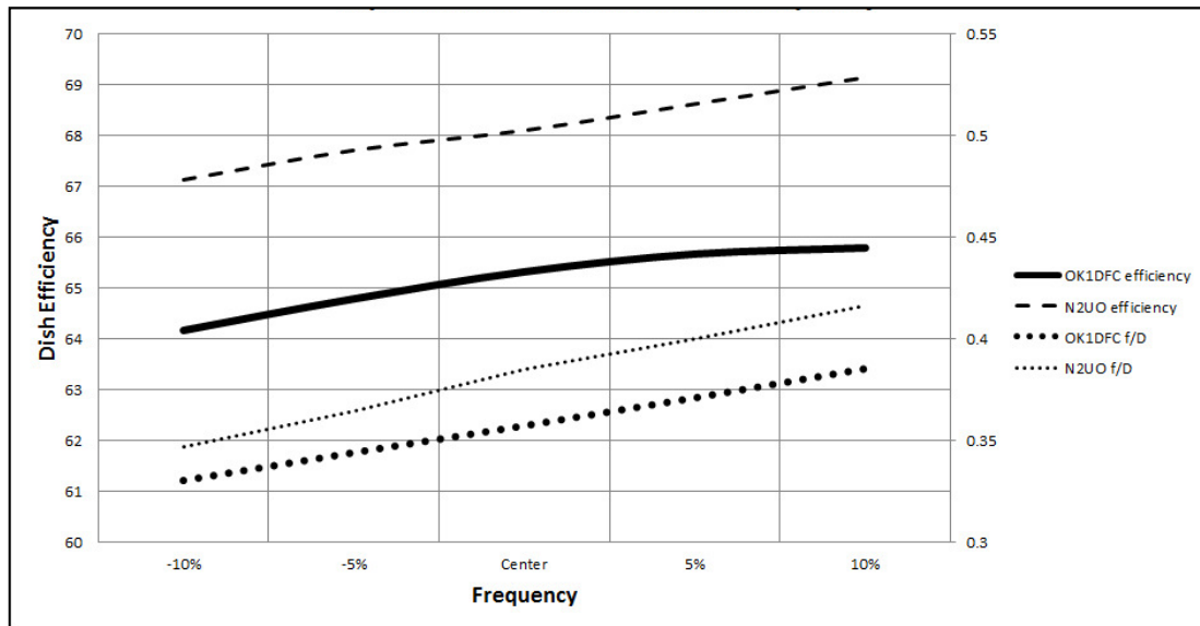
Figure 8: Antenna performance over frequency range
