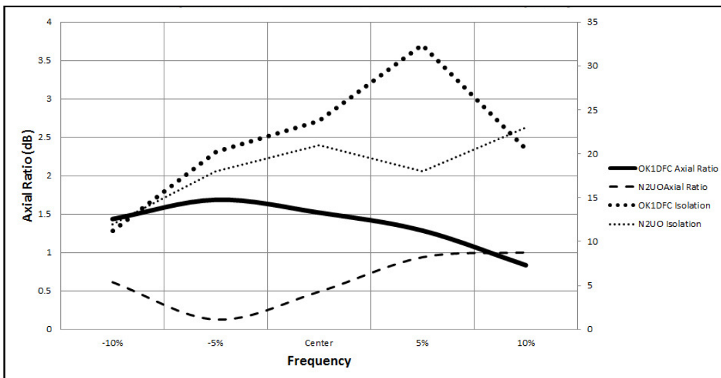
Figure 7: Axial Ratio and Isolation over frequency range
