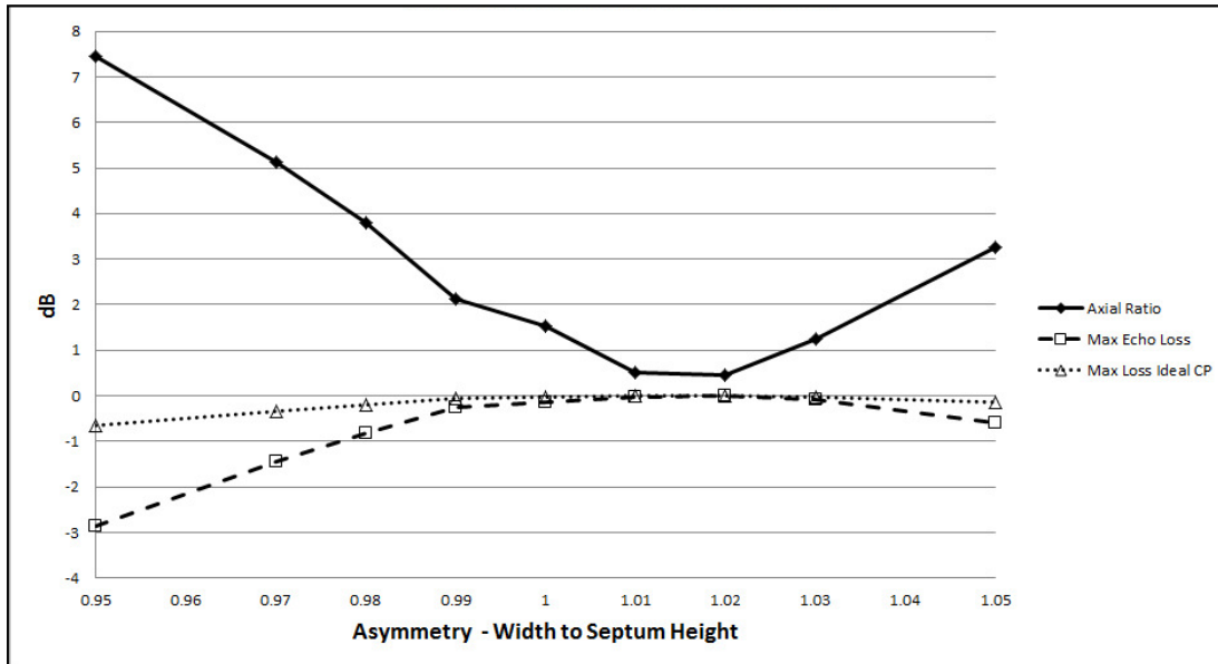
Figure 9: Effect of waveguide asymmetry on OK1DFC septum feed
