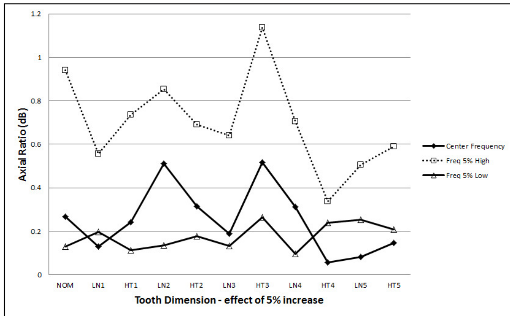
Figure 5: N2UO septum feed, sensitivity to tooth dimension
